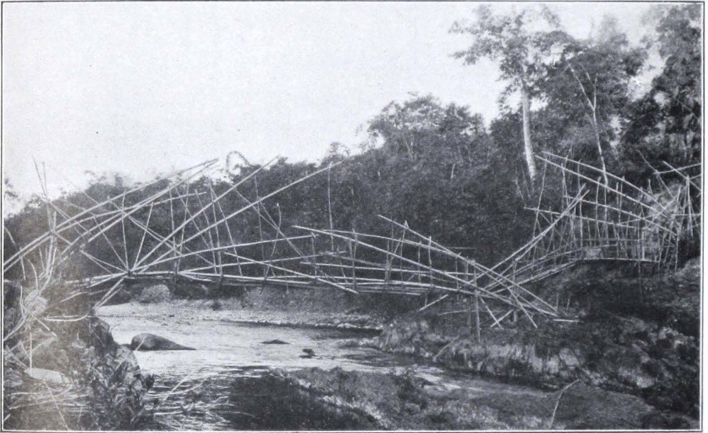
A KACHA NAGA (LYENGMAI) BRIDGE ON THE CANTILEVER PRINCIPLE
